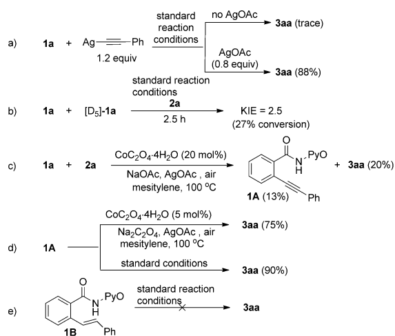
Scheme 1. Control experiments.
